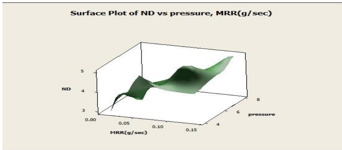
Fig. 5 Surface plot of ND vs pressure, MRR
