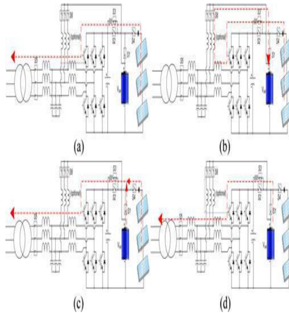
Fig3. All operation modes of the RSC. (a) Mode 1—PV to grid. (b) Mode 2—PV to battery. (c) Mode 3—PV/battery to grid. (d) Mode 4—battery to grid.
