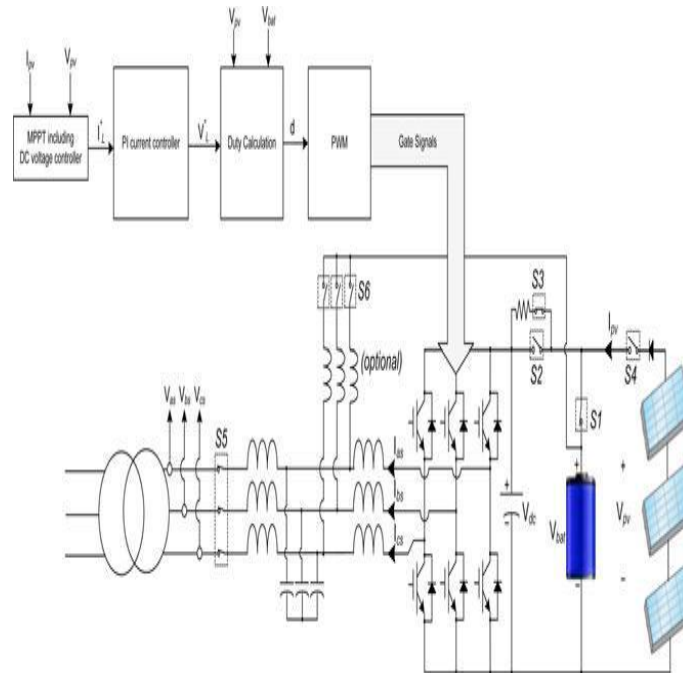
Fig7. Overall control block diagram of the RSC in the dc/dc operation
