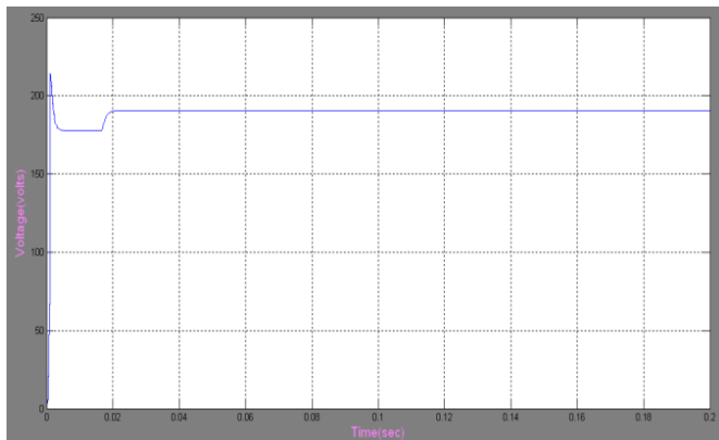
(a) PV output voltage
