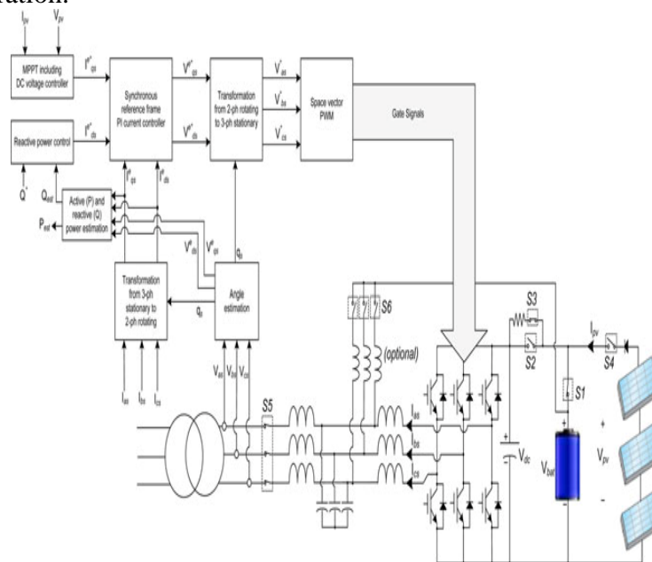
Fig.6. Overall control block diagram of the RSC in the dc/ac operation.
