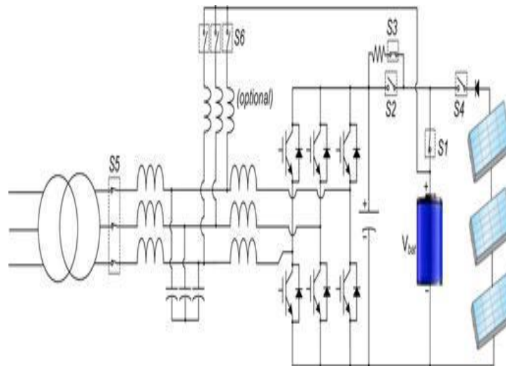
Fig2. Schematic of the proposed RSC circuit.
