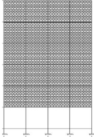
Case3- Building with Open Ground Story
