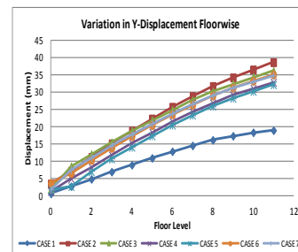
Graph 1: Zone II, Y-direction
