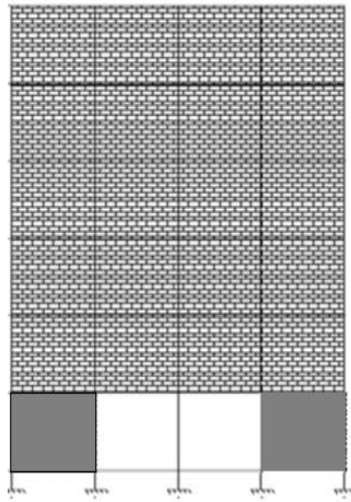
Case5- OGS with Corner Shear wall
