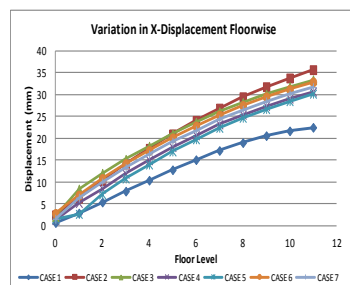
Graph 3 : Zone III, X-direction
