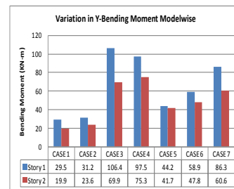
Graph 12 : Zone III, Y-direction
