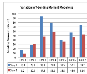
Graph 10 : Zone II, Y-direction
