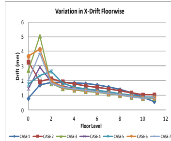
Graph 23 : Zone V, X-direction
