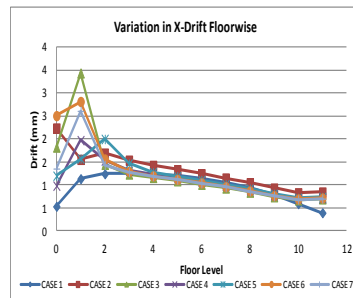
Graph 21 : Zone IV, X-direction
