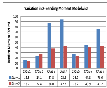
Graph 9 : Zone II, X-direction
