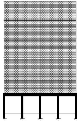
Case4- OGS with Stiffer Column (MF 2.5)
