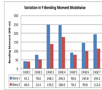
Graph 16 : Zone V, Y-direction
