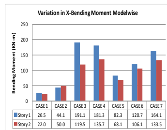
Graph 11 : Zone III, X-direction
