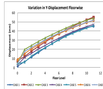
Graph 6: Zone IV, Y-direction
