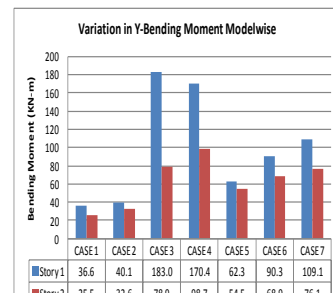
Graph 14 : Zone IV, Y-direction
