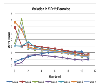
Graph 20 : Zone III, Y-direction
