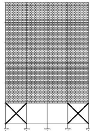
Case6- OGS with Cross Bracing
