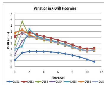
Graph 17 : Zone II, X-direction
