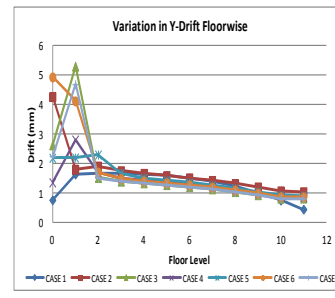
Graph 22 : Zone IV, Y-direction
