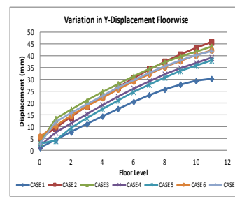
Graph 4 : Zone III, Y-direction
