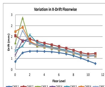
Graph 19 : Zone III, X-direction
