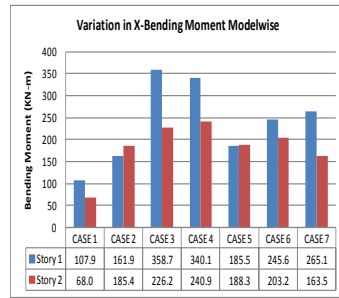
Graph 15 : Zone V, X-direction
