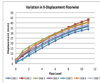
Graph 5 : Zone IV, X-direction
