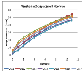
Graph 7 : Zone V, X-direction
