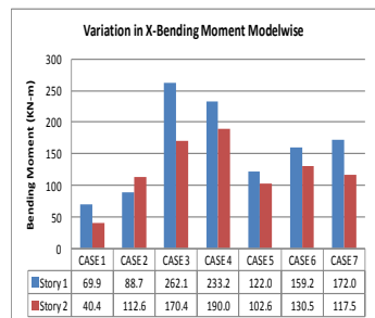
Graph 13 : Zone IV, X-direction
