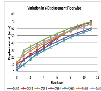
Graph 8 : Zone V, Y-direction
