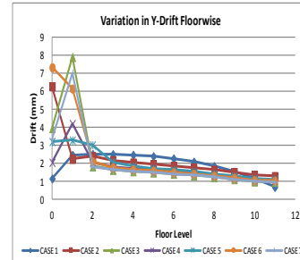
Graph 24 : Zone V, X-direction
