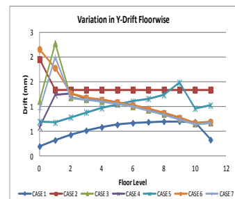
Graph 18 : Zone II, Y-direction
