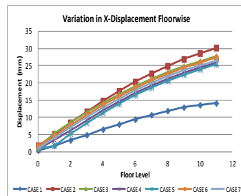
Graph 1 : Zone II, X-direction
