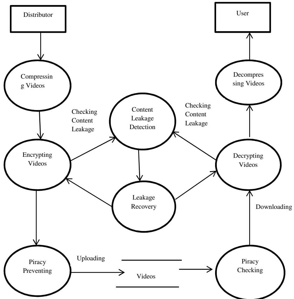
Figure 2. Dataflow Diagram for Overall Design
