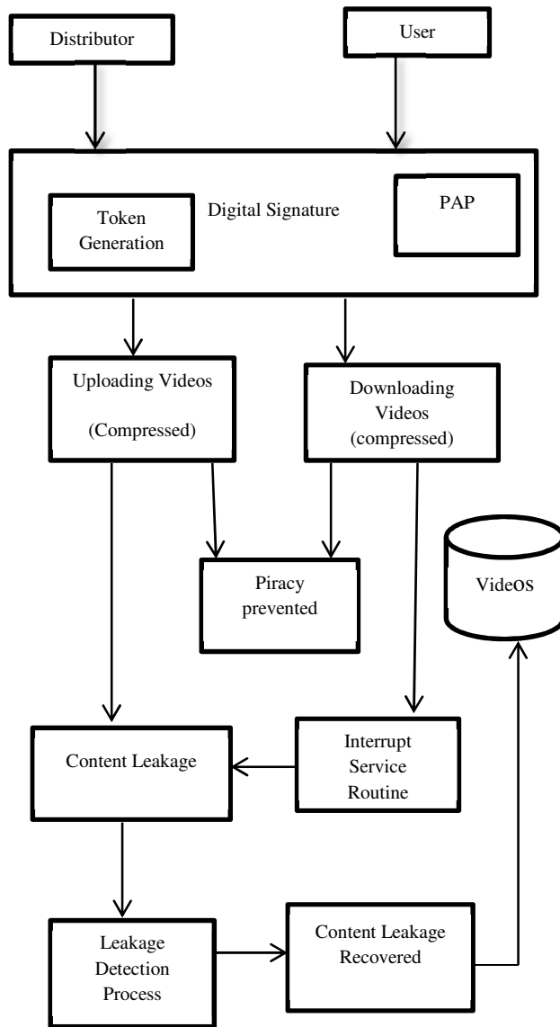
Figure 1. Framework for Content Leakage and Piracy Prevention
